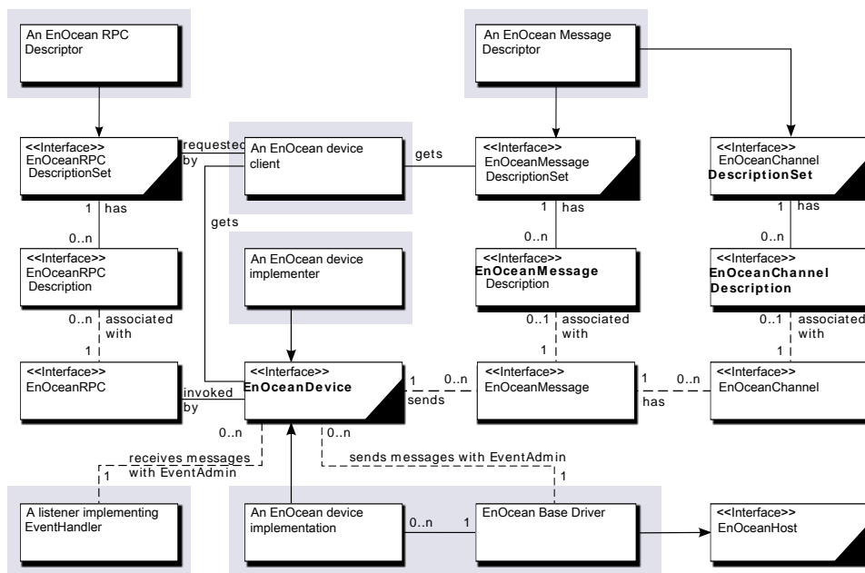
Figure 139.1 EnOcean Service Specification class diagram.
