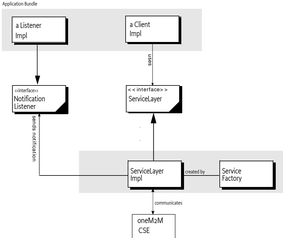
Figure 153.1 Entity overview of Service Layer API for oneM2M
