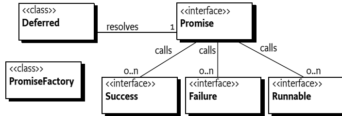
Class diagram of org.osgi.util.promise
