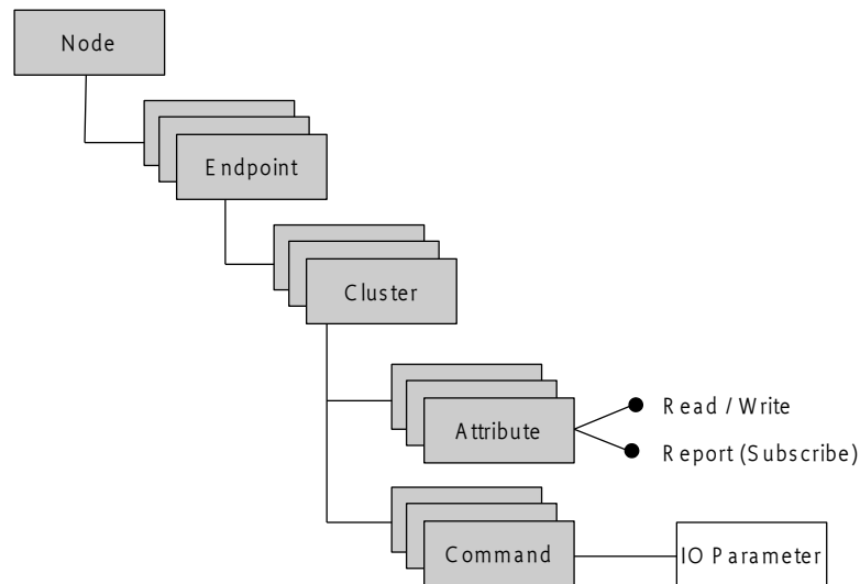
Figure 149.5 ZigBee Cluster Library model
