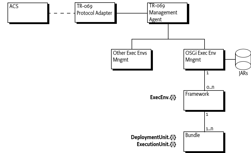
Figure 155.1 Management Agent Architecture
